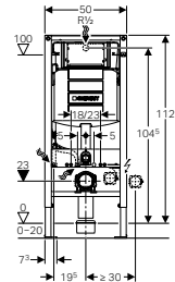
Kombifix element with UP320, front actuation, thickness 12 cm.
