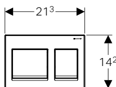
Geberit actuator plate Alpha 15 for dual flush
