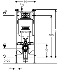
Geberit Duofix element for wall-hung WC, 114 cm, with Alpha concealed cistern 8 cm
