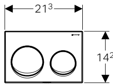
Geberit actuator plate Alpha 10 for dual flush
