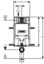
Geberit Kombifix element for wall-hung WC, 109 cm, with Alpha concealed cistern 8 cm
