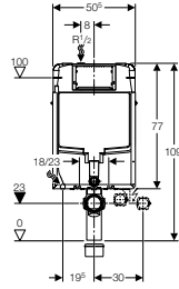
Kombifix element, front actuation, thickness 8 cm.
