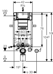
Kombifix element with UP320, front actuation, thickness 12 cm.
